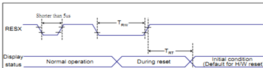
Figure 10 Reset Timing
