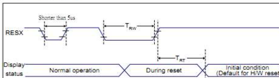
Figure 10 Reset Timing
