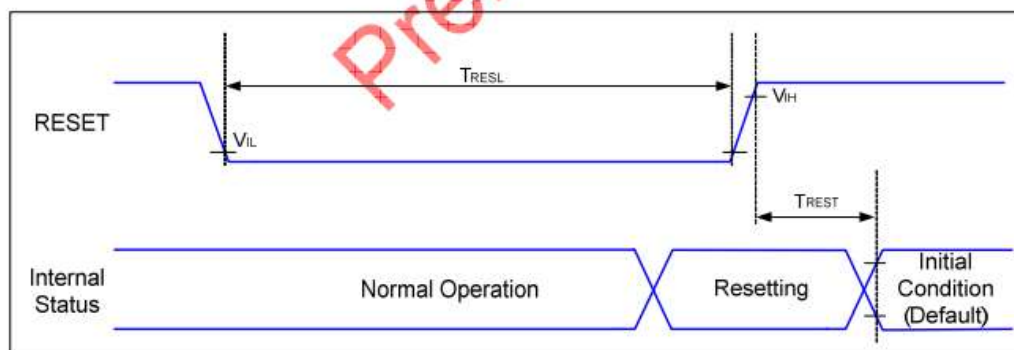
Figure 51 Reset Timing
