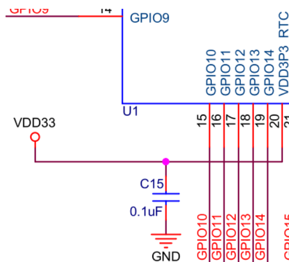
Fig. 5: ESP32-S3 Schematic for RTC Power Supply Pin
