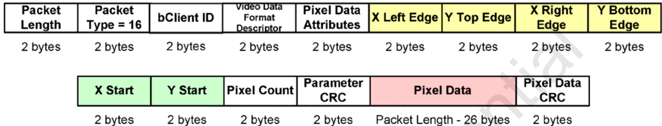
Figure 6.3.3.2.1 Video stream packet
