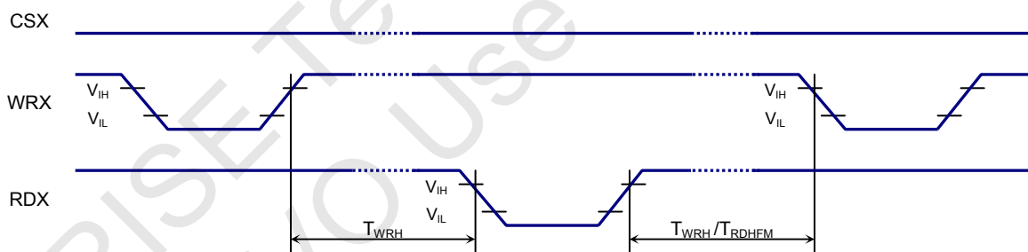
Fig. 7.3.3.4 Write to read and Read to write timing
