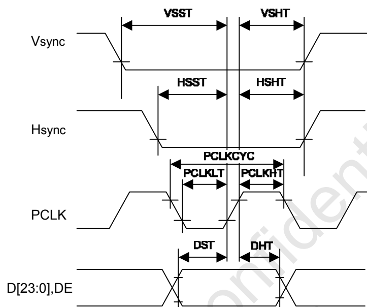
Figure 7.3.5.1 AC Timing Characteristics, RGB Interface
