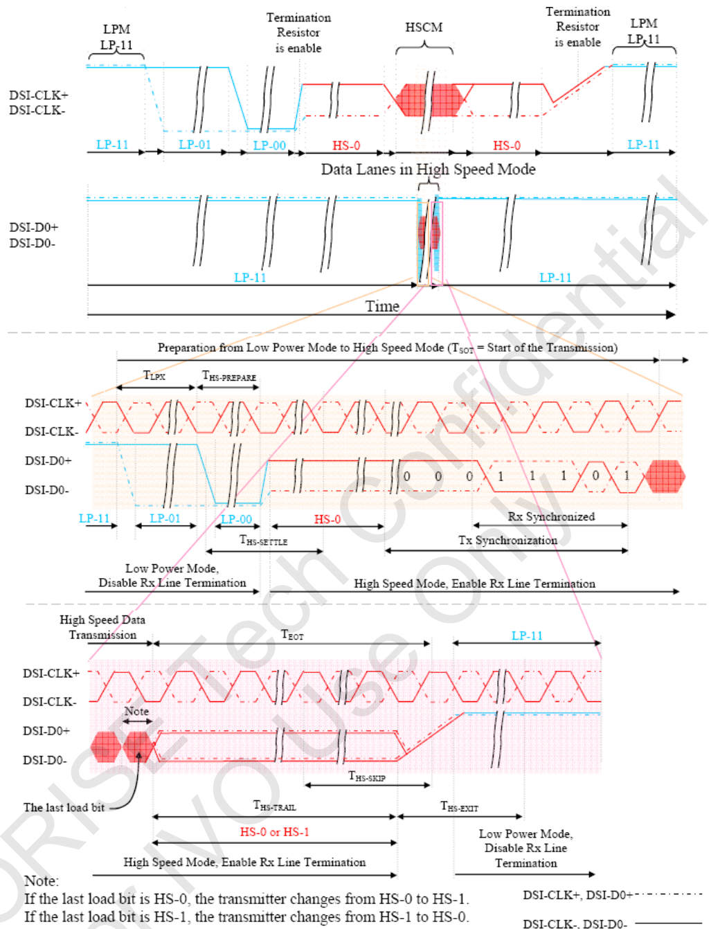
Figure 6.2.2.2.9. High speed clock burst
