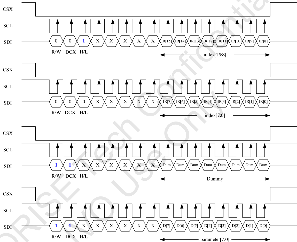
Figure 6.7.2.1 SPI Protocol for register read mode
