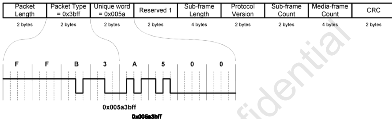
Figure 6.3.3.1.1 Sub frame header packet format
