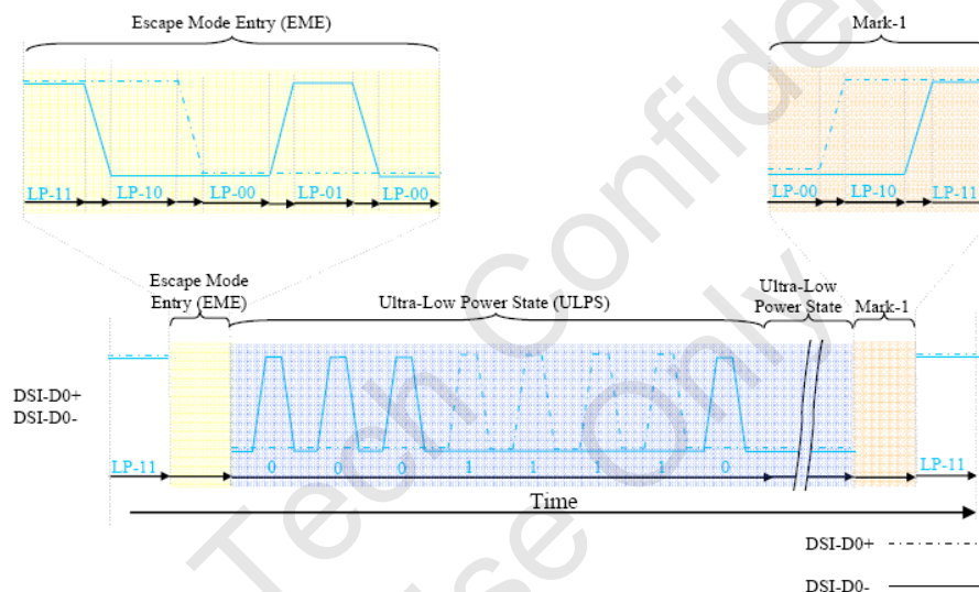
Figure 6.2.3.2.5. Ultra-low power state (ULPS)
