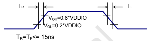
Fig. 7.3.3.2 Rising and Falling timing for Input and Output signal
