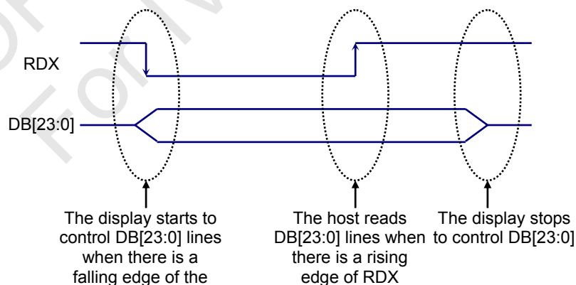
Fig. 6.5.2.1 8080-Series RDX Protocol
