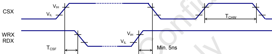
Fig. 7.3.3.3 Chip selection (CSX) timing
