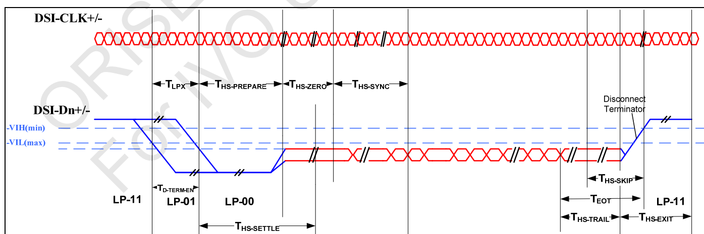
Fig. 7.3.1.3.1: High Speed Data Transmission Bursts
