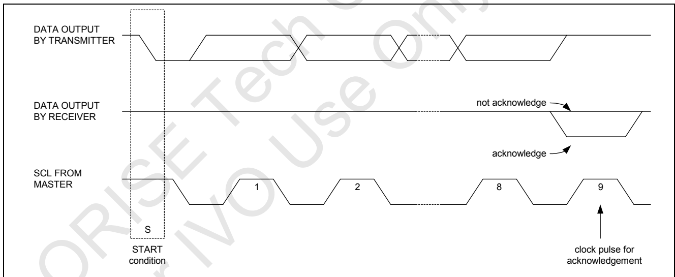
Figure 6.6.1.4 Acknowledgement on the I 2 C-bus.
