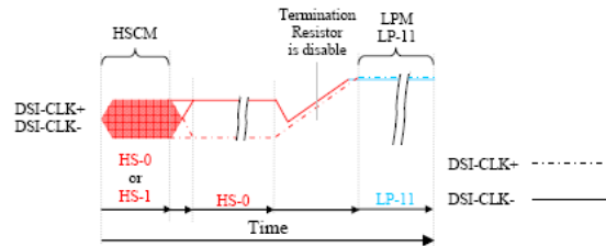
Figure 6.6.2.2.3. From HSCM to LPM
