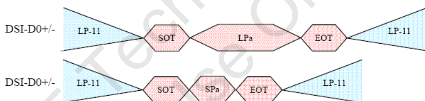
Figure 6.2.3.3.3. Single packet in HSDT
