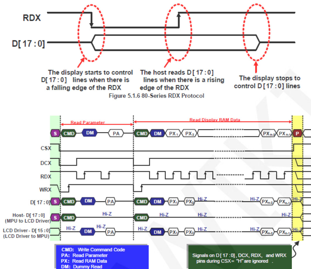
Figure 5.1.7 80-Series Parallel Bus Protocol for Register or RAM Read
