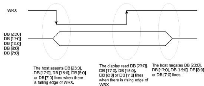
Figure 1: DBI Type B Write Cycle
