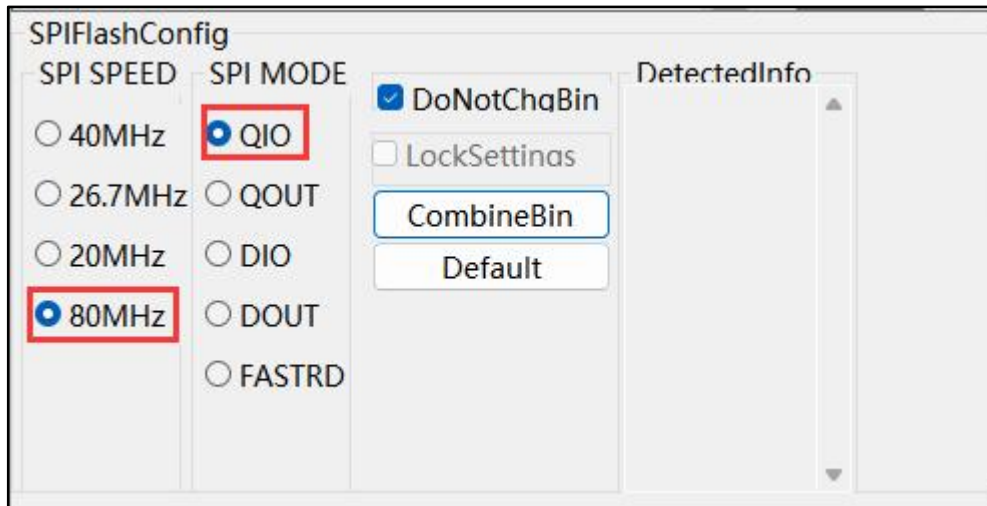
Picture 6 flash_download_tool setting 2
