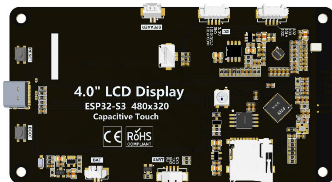
Figure 2.1 Rear view of 4.0-inch ESP32-S3 display module
