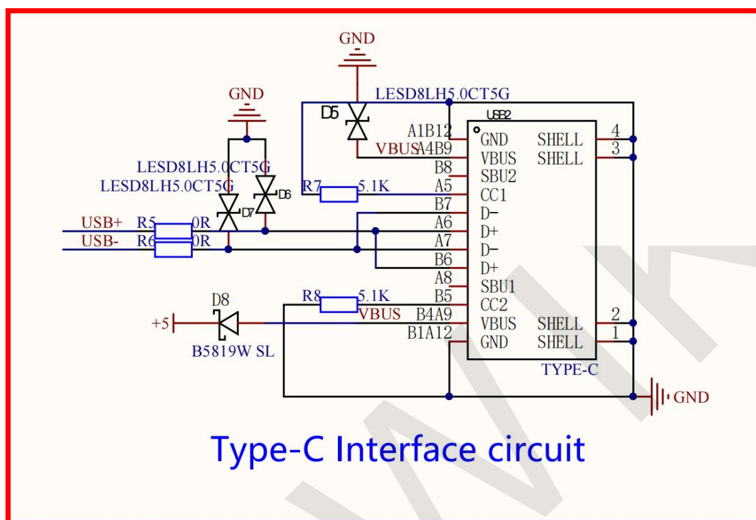
Figure 3.5 Type-C interface circuit
