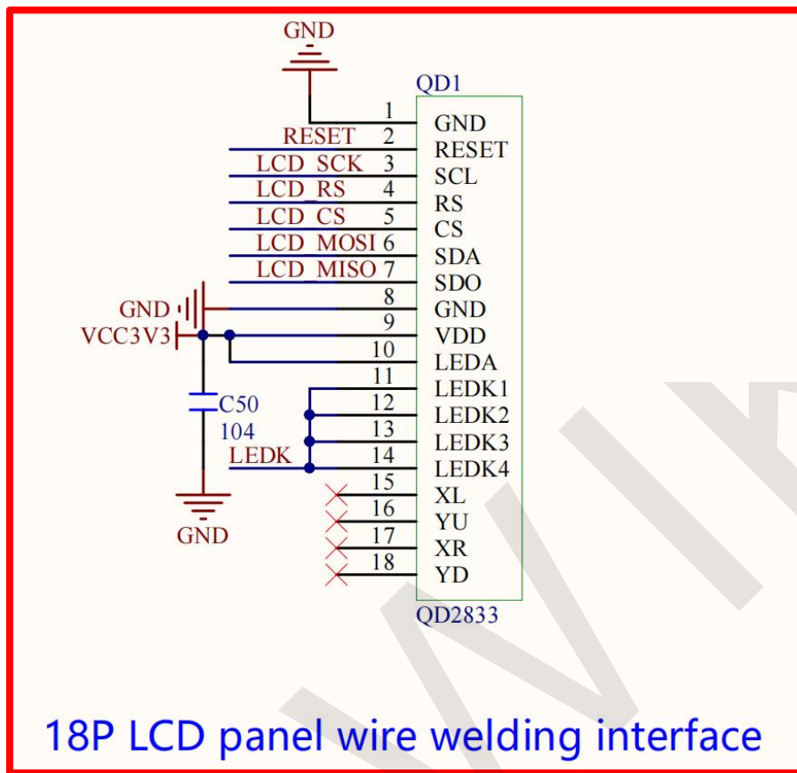
Figure 3.15 18P LCD panel wiring welding interface
