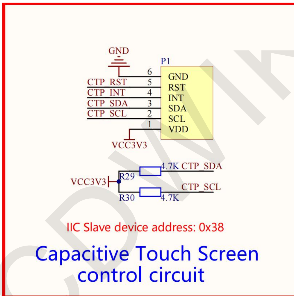
Figure 3.8 Capacitive touch screen interface circuit
