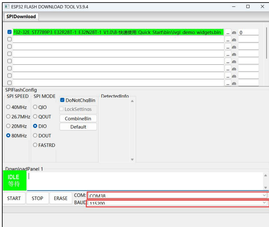
Figure 9 flash_download_tool Setup 3
