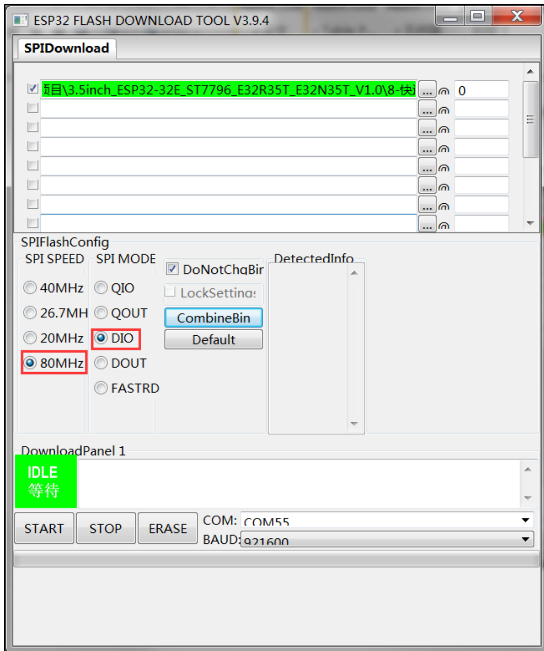
Figure 8 flash_download_tool Setup 2
