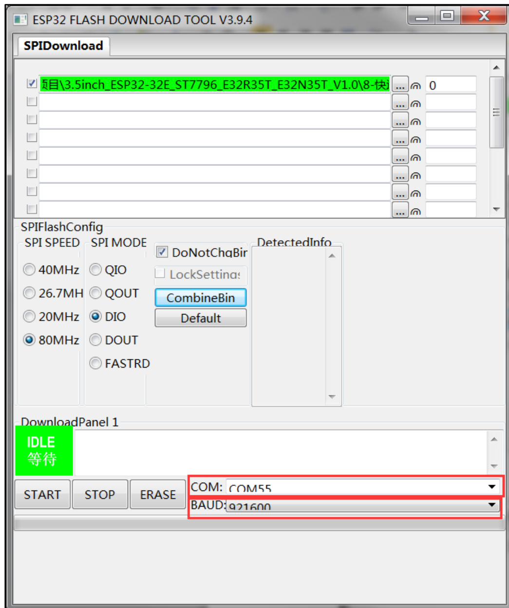
Figure 9 flash_download_tool Setup 3
