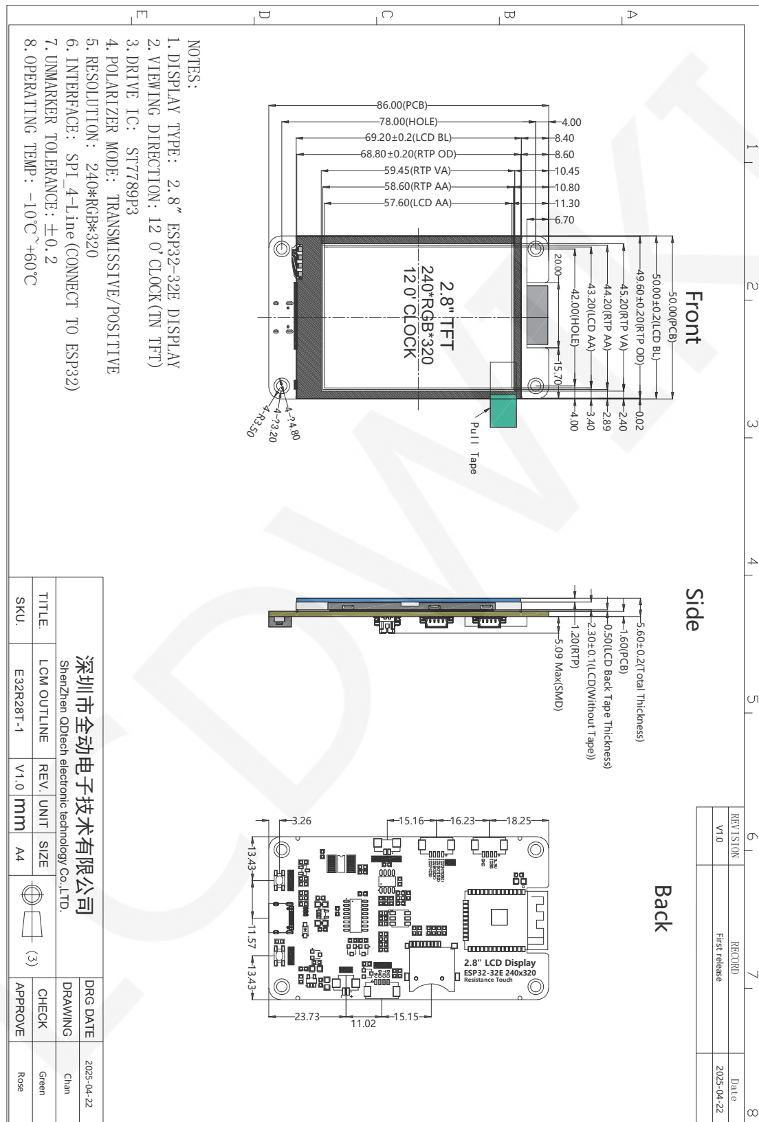
Figure 5.1 Dimensions of E32R28T-1
