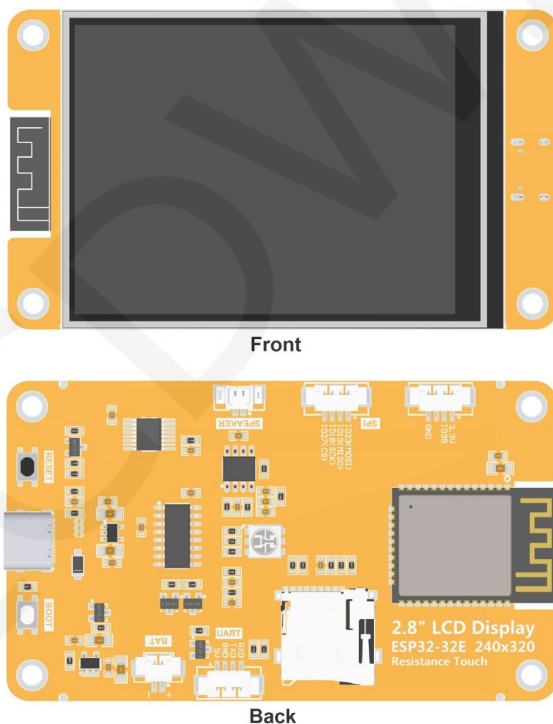
Figure 1.1 E32R28T-1 product diagram
