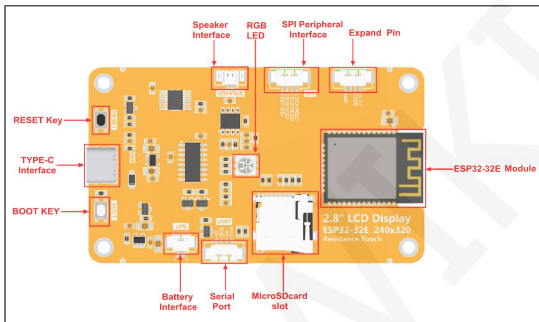
Figure 4.1 product interface diagram
