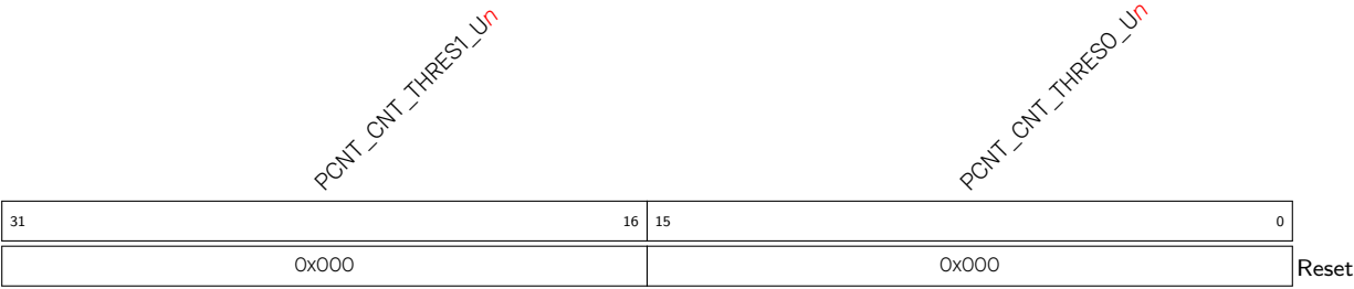
Register 17.2. PCNT_Un_CONF1_REG ( n : 0-7) (0x4+0x0C* n )
