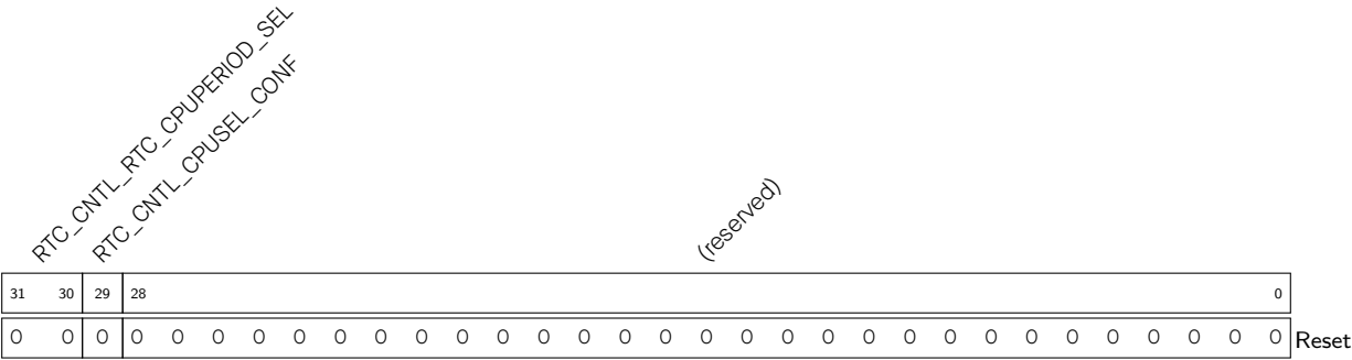
Register 31.23. RTC_CNTL_CPU_PERIOD_CONF_REG (0x0068)
