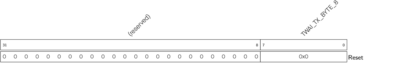
Register 21.13. TWAI_DATA_8_REG (0x0060)
