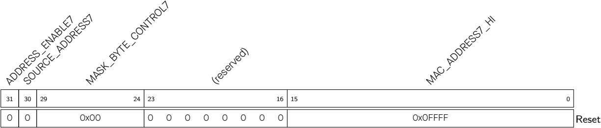
Register 10.41. EMACADDR7HIGH_REG (0x107C)
