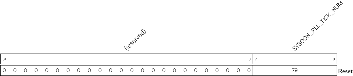
Register 3.3. SYSCON_PLL_TICK_CONF_REG (0x0008)
