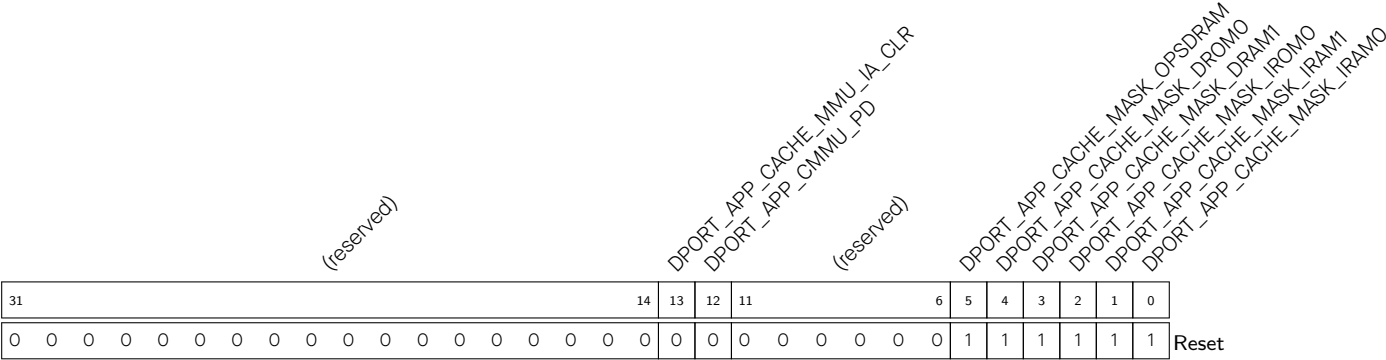
Register 5.13. DPORT_APP_CACHE_CTRL1_REG (0x05C)
