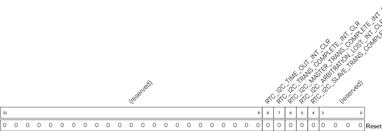
Register 30.13. RTC_I2C_INT_CLR_REG (0x024)
