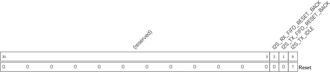
Register 12.35. I2S_STATE_REG (0x00bc)
