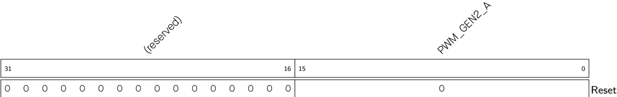
Register 16.45. PWM_GEN2_TSTMP_A_REG (0x00b0)
