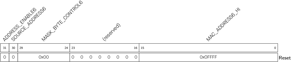
Register 10.39. EMACADDR6HIGH_REG (0x1074)
