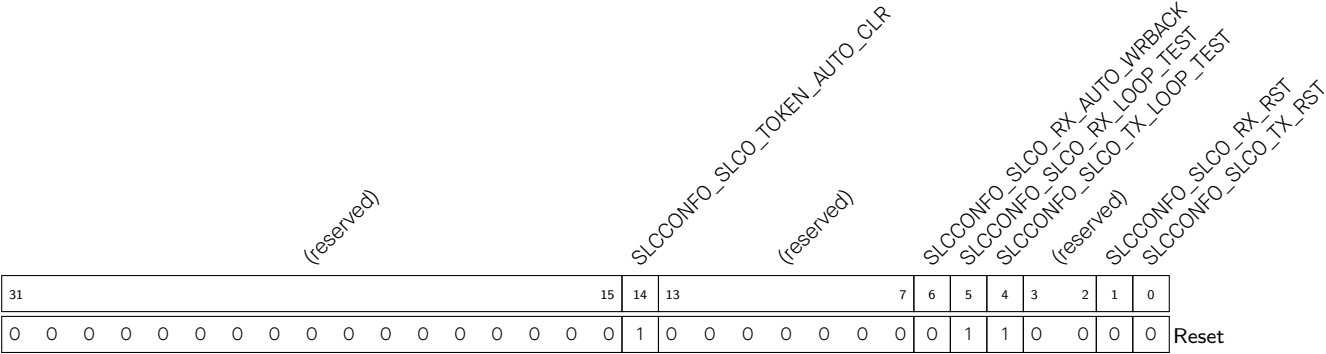
Register 8.1. SLCCONFO_REG (0x0)
