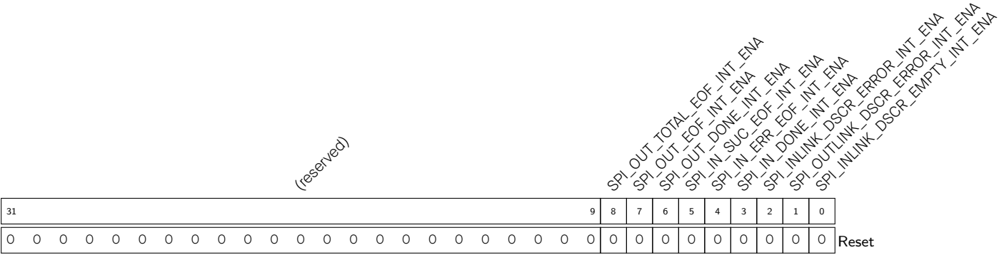
Register 7.29. SPI_DMA_INT_ENA_REG (0x110)
