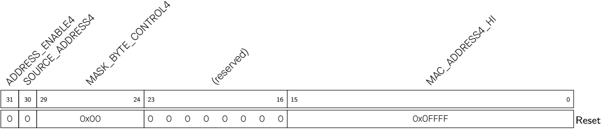
Register 10.35. EMACADDR4HIGH_REG (0x1064)
