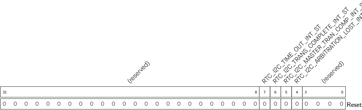
Register 30.15. RTC_I2C_INT_ST_REG (0x02c)
