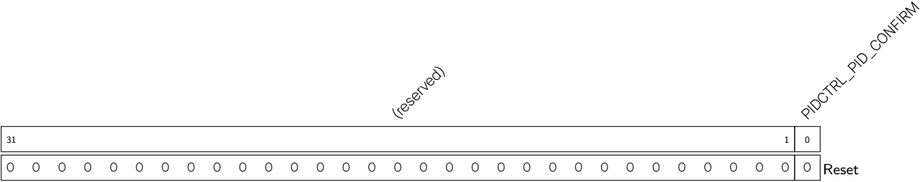
Register 28.14. PIDCTRL_PID_CONFIRM_REG (0x04C)
