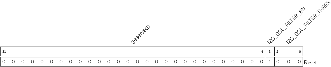
Register 11.19. I2C_SCL_FILTER_CFG_REG (0x0050)
