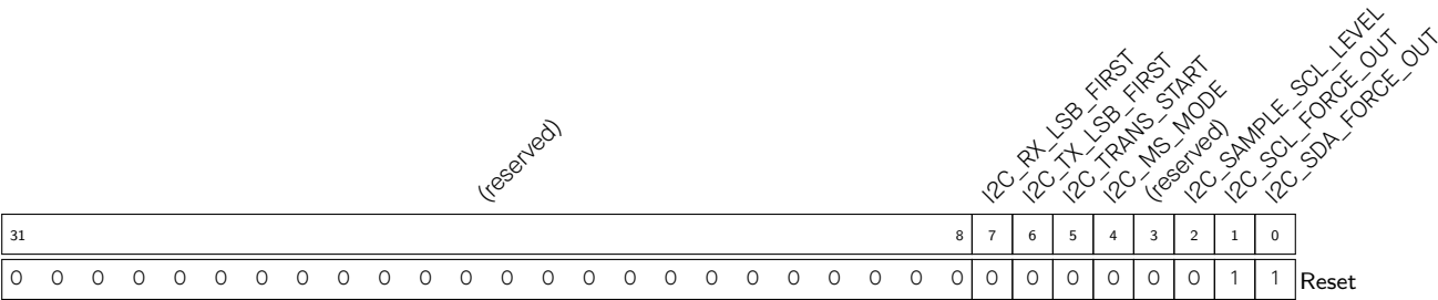
Register 11.2. I2C_CTR_REG (0x0004)
