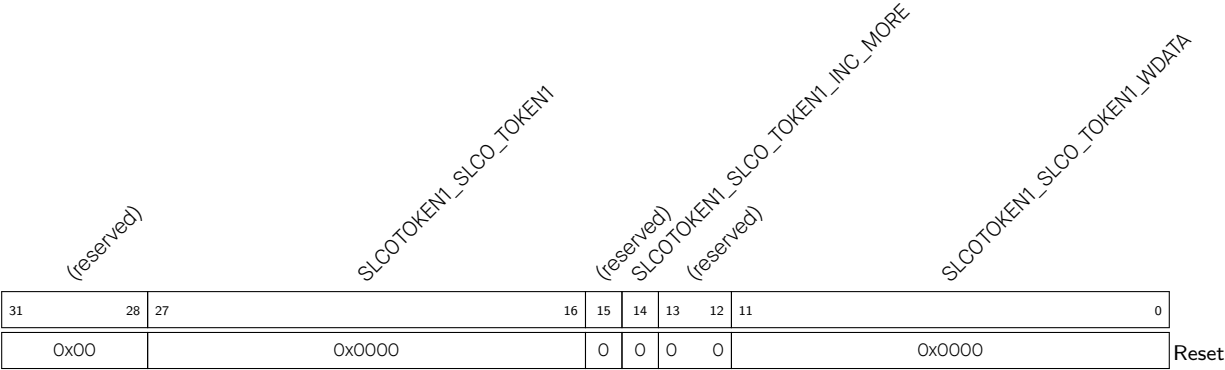
Register 8.9. SLCOTOKEN1_REG (0x54)
