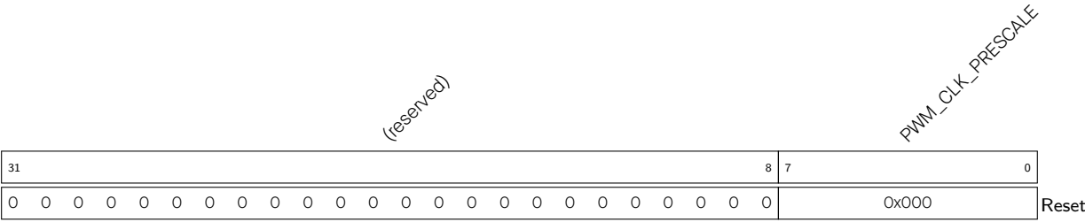
Register 16.1. PWM_CLK_CFG_REG (0x0000)
