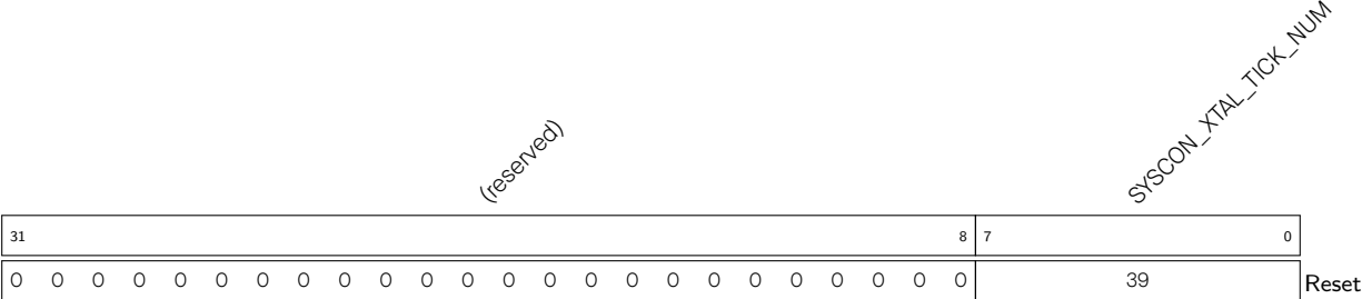
Register 3.2. SYSCON_XTAL_TICK_CONF_REG (0x0004)
