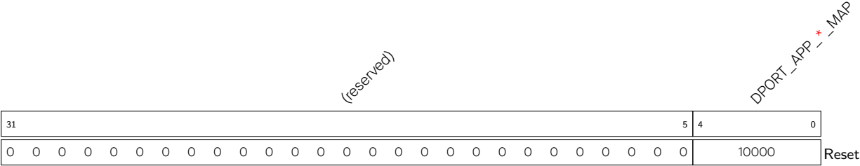
Register 5.159. DPORT_APP_CACHE_IA_INT_MAP_REG (0x328)
