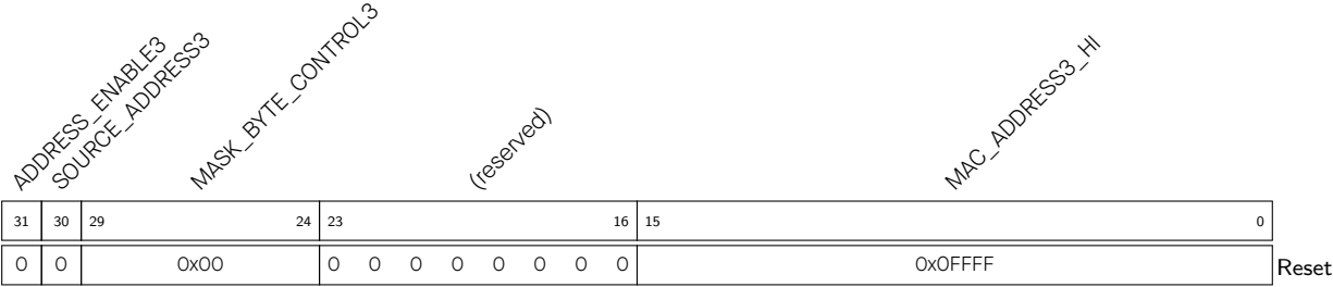
Register 10.33. EMACADDR3HIGH_REG (0x1058)
