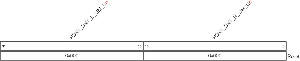
Register 17.3. PCNT_Un_CONF2_REG ( n : 0-7) (0x8+0x0C* n )
