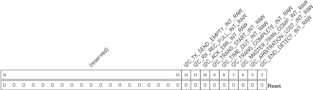
Register 11.8. I2C_INT_RAW_REG (0x0020)
