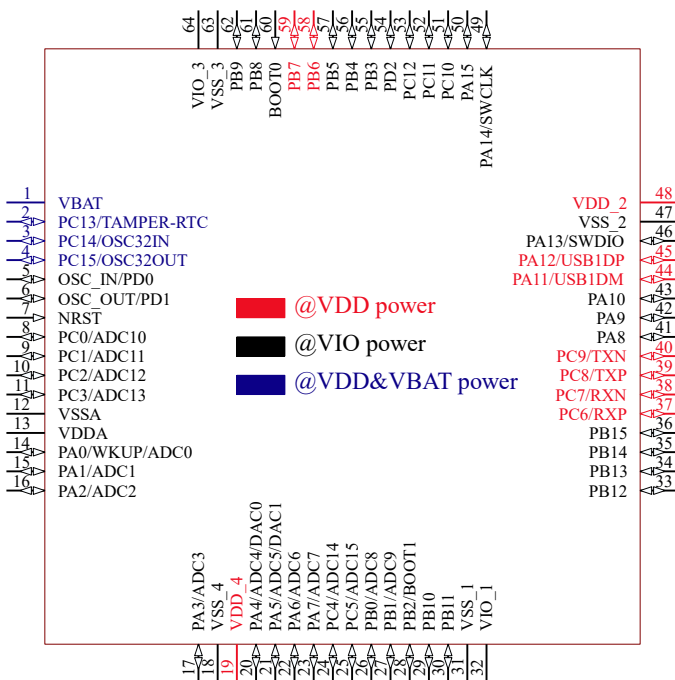
CH32F203RCT6
