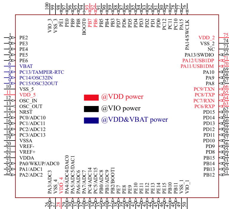
CH32F203VCT6
