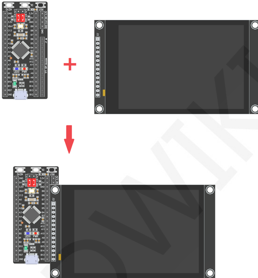
Figure 2: Module Inline CH32F203C8T6 Development Board
