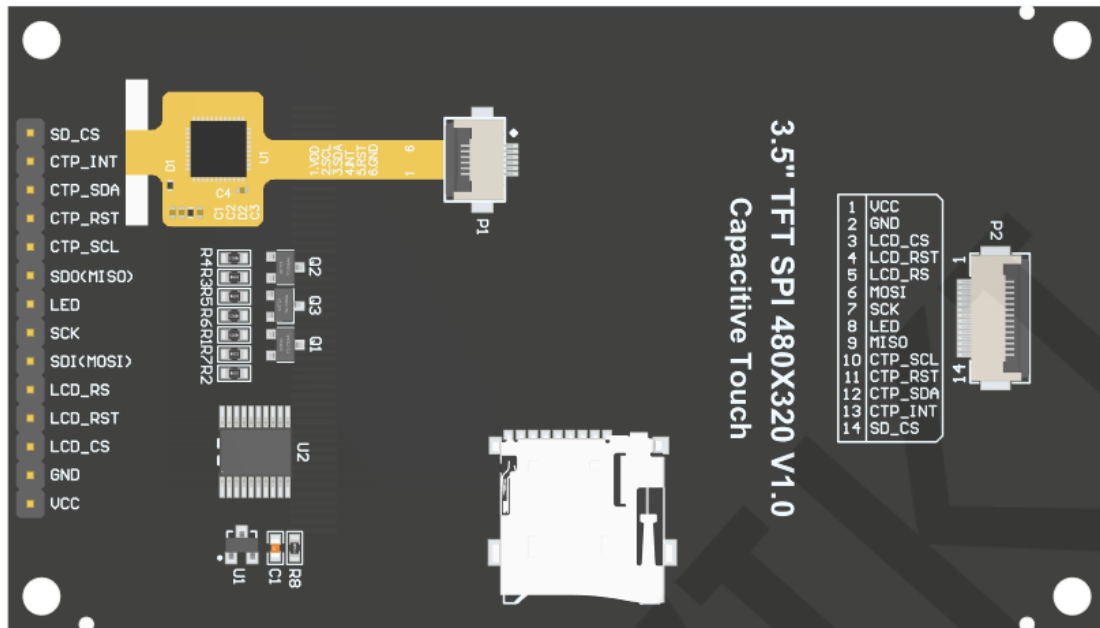
Figure 3 Module Back Pins
