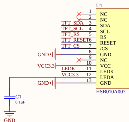
IPS屏13Pin FPC接口
